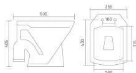
COCO - S Water Closet L 505 W 355 H 405 MRP 5200/-
