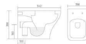
TATA - S&P Water Closet L 542 W 368 H 388 MRP 7500/-
