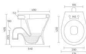
CLASSIC - S Water Closet L 540 W 375 H 405 MRP 2400/- WITHOUT SEAT COVER
